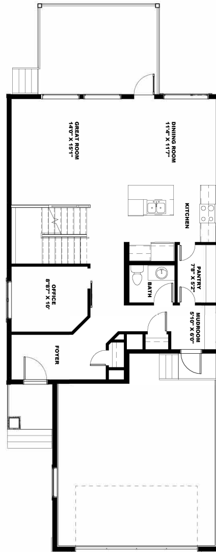
MAIN FLOOR 1,016 sq. ft.
